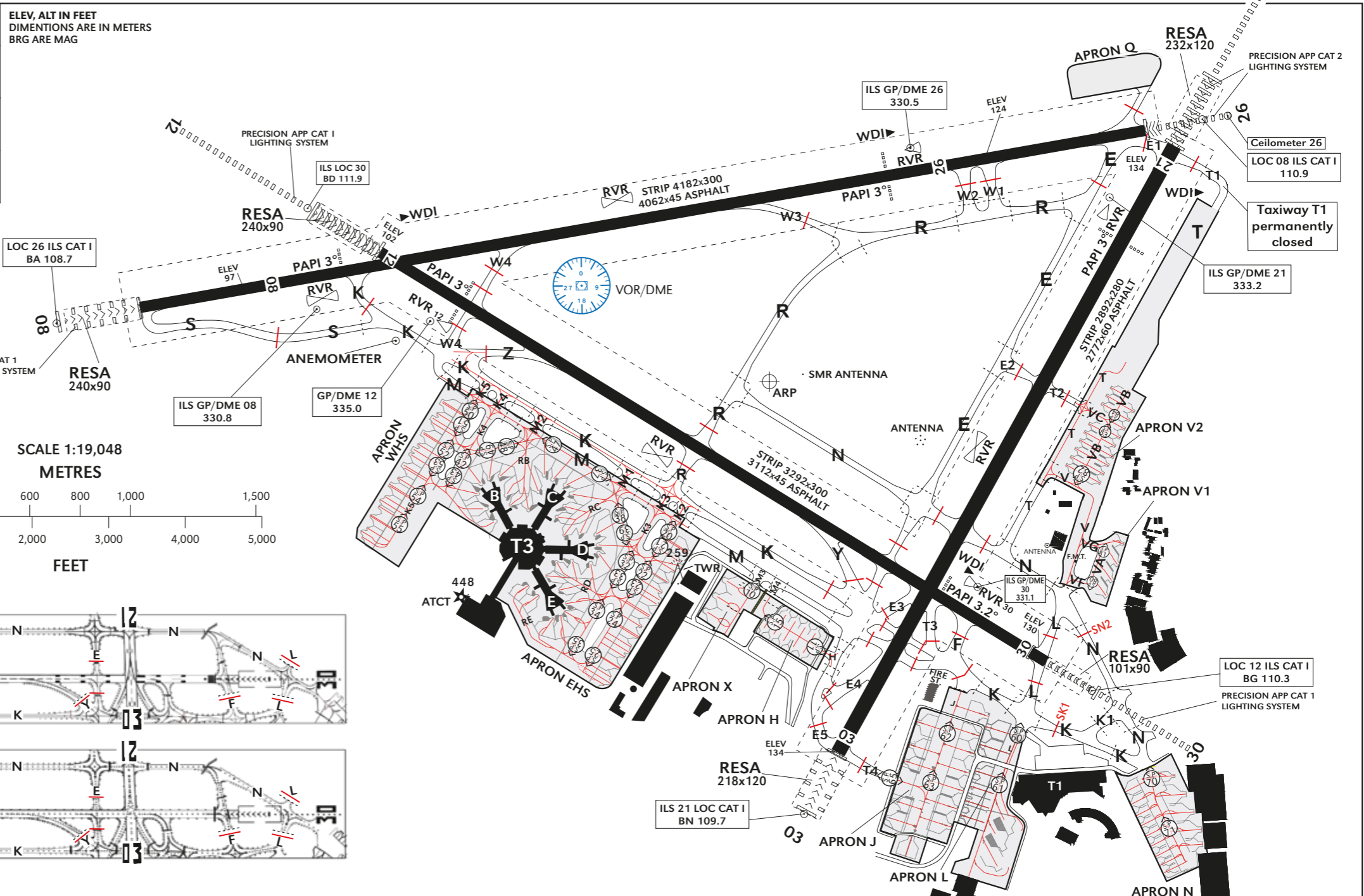
MARKING AIDS RWY 03/21 AND EXIT TWY
